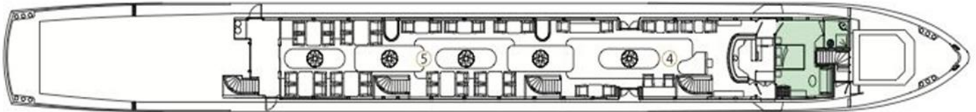
Saloon Deck
